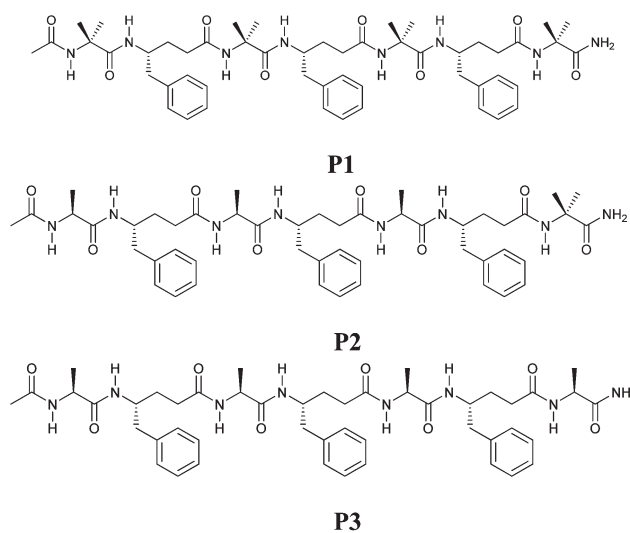
Scheme 2 \alpha/\gamma^4 -Hybrid peptides P1 , P2 and P3 synthesized using solid phase peptide synthesis.
